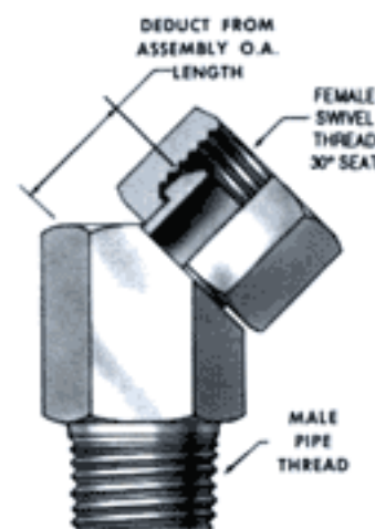
LENZ MEX-UAD MALE 45° UNION ELBOW SWIVEL ADAPTER Male Pipe To Female NPSM Swivel
