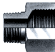
PRC-B — Pipe Reducing Connector Tapered Male Pipe Thread One End Tapered Female Pipe Thread Other End
