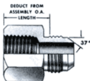
LENZ 3255 FEMALE ADAPTER Female Pipe To J.I.C. Thread
