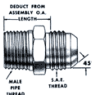
LENZ 5105 MALE ADAPTER
