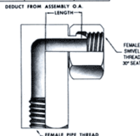
LENZ FE-UAD FEMALE UNION ELBOW SWIVEL ADAPTER Female Pipe To Female NPSM Swivel
