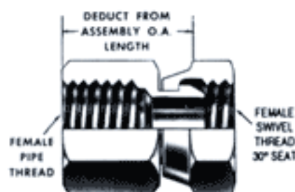
LENZ F-UAD FEMALE UNION SWIVEL ADAPTER Female Pipe To Female NPSM Swivel
