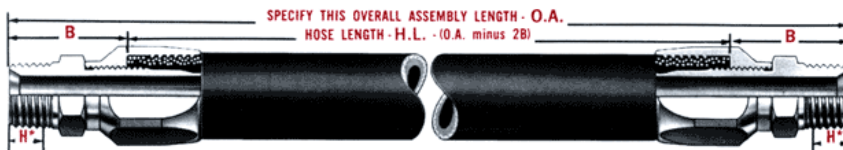
SHOWN ABOVE - AL ASSEMBLIES \frac{1}{2} " I.D. HOSE SIZE and LARGER (STEEL FITTINGS)
