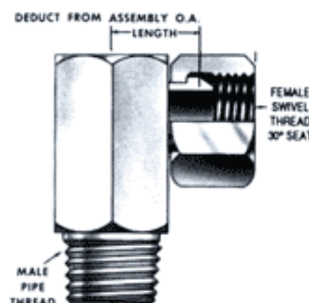
LENZ ME-UAD MALE UNION ELBOW SWIVEL ADAPTER Male Pipe To Female NPSM Swivel
